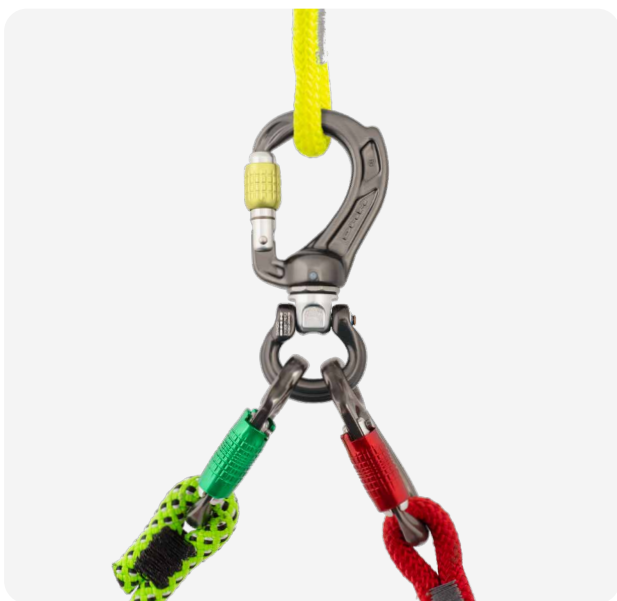
› Director Swivel Boss Screwgate with Compact Shackle L - Bow shape (A642BS) configured with two Director Captive Eye (A653 and A657)
