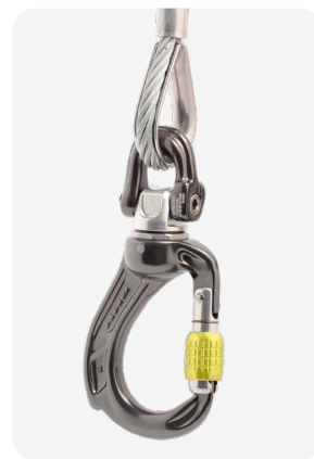
› Director Swivel Boss Screwgate with Compact Shackle S - D shape (A662SS)
